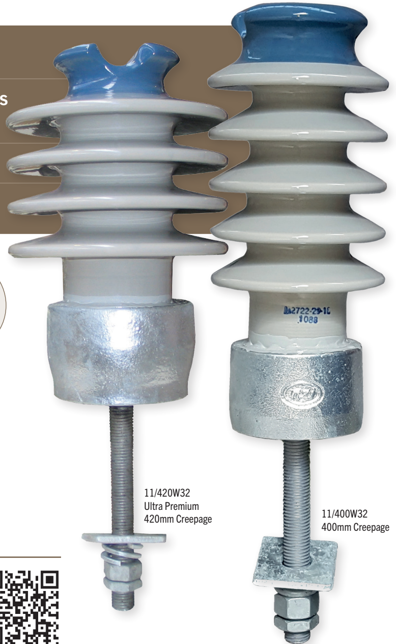
32mm Groove with Radio Silent Glaze
